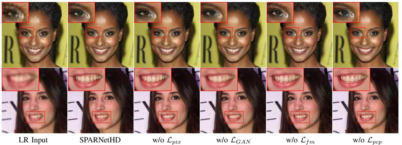
Fig. 12: Ablation study of losses used in SPARNetHD on the synthetic dataset CelebAHQ-Test (first row) and real dataset CelebA-TestN (second row). Better zoom in to see the details.
