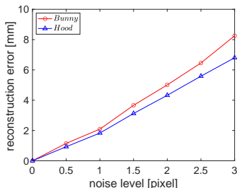
Fig. 12. Reconstruction results under different quantization noise.
