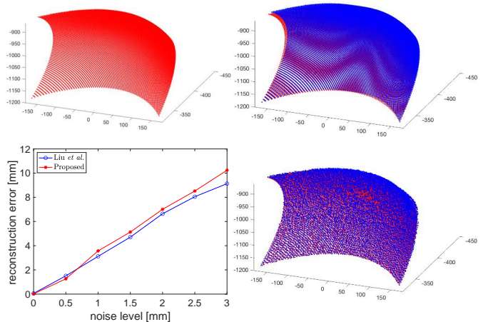
Fig. 13. Comparison with a fully calibrated method of Liu et al. [15]. Upper left: ground truth. Lower left: RMS reconstruction errors. Upper right ([15]) & lower right (ours): reconstruction (blue) against ground truth (red) under \sigma = 2.0 . Our uncalibrated approach achieves comparable accuracy with that of the fully calibrated method in [15].
