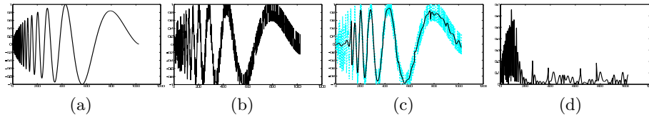
Fig. 1. In (a), it shows the original Doppler function. In (b), it shows the Doppler function contains 10dB noise. In (c), it shows the denoised signal in black solid line compare with the noisy signal in cyan dotted line. In (d), it shows the relative square error with peak value 0.67 and average value 0.153.
