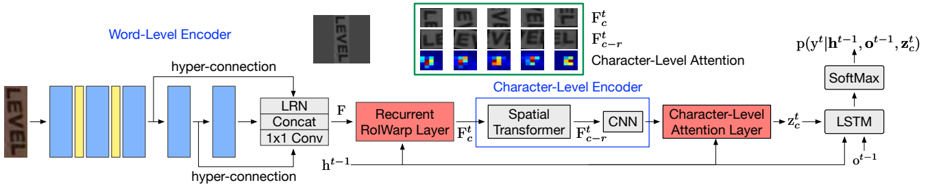
Figure 2: Overall architecture of the Char-Net. Blue and yellow rectangles in the word-level encoder represent the convolutional blocks and the max-pooling layers, respectively. Three convolutional feature maps from different levels of the CNN are normalised (local response normalization), concatenated and dimension-reduced ( 1 \times 1 convolution) to produce the feature map \mathbf{F} . Two red rectangles denote the two layers of the hierarchical attention mechanism. The corresponding image patches of \mathbf{F}_c^t and \mathbf{F}_{c-r}^t together with the character-level attentions are shown in the green rectangle.
