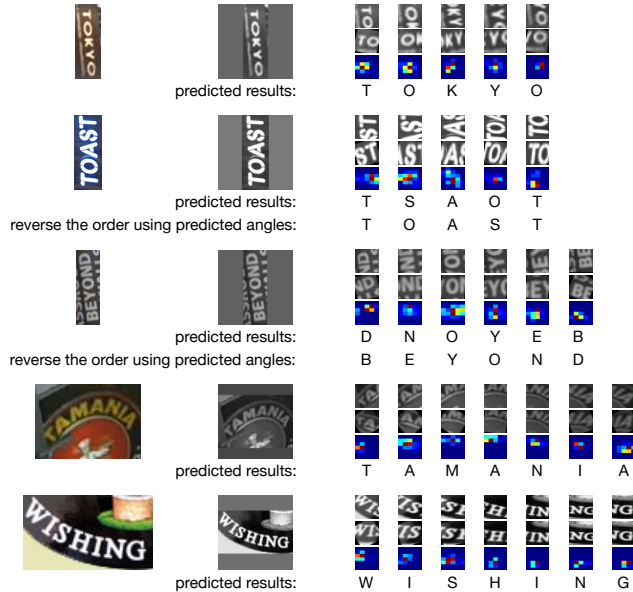
Figure 4: Some examples of largely distorted scene text being recognized by our Char-Net. The first and second columns are the original images and the square images for training, respectively. The corresponding image patches of the attended and rectified character feature regions together with the character-level attentions are shown in the third column. Note that in order to get the correct predictions of the second and third images, we reverse the order of the predicted characters according to their rotation angles.
