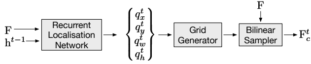
Figure 3: The detailed structure of the recurrent RoIWarp layer.
