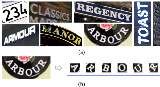
Figure 1: (a) Some examples of scene text suffering from different kinds of distortion. (b) A text along a curve can be considered a sequence of individually rotated characters.
