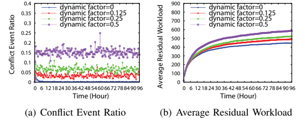
Figure 7. SPIRA algorithm over different dynamic environment
