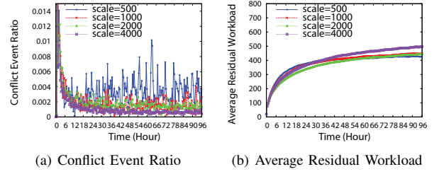
Figure 6. Scalability of SPIRA algorithm
