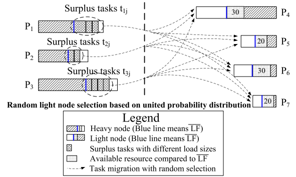
Figure 1. Decentralized load balancing can be viewed as Bernoulli trial
