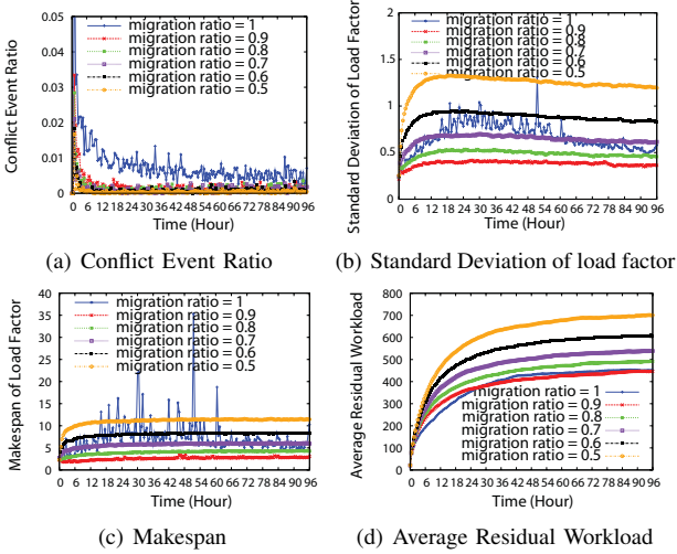
Figure 5. SPIRA algorithm under different load migration ratios
