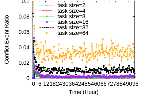
Figure 3. Conflict probability of SPIRA with various task sizes
