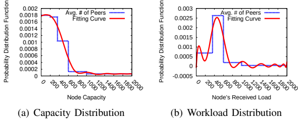
Figure 2. Capacity and workload distribution among nodes
