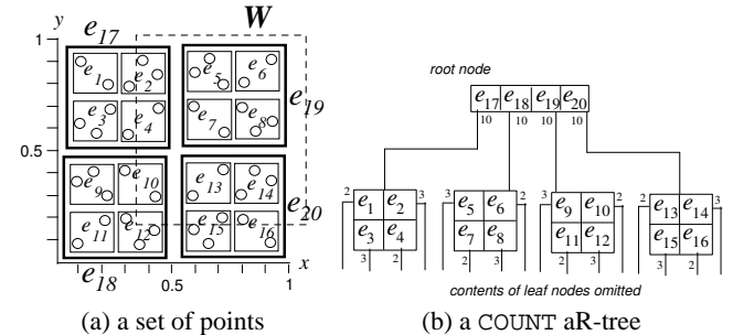
Figure 2: aR-tree example
