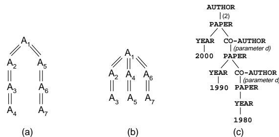
Figure 14: Twig queries used in the experiments
