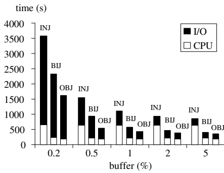
Figure 15: The Effect of Buffer Size, |P| = |Q| = 200K , Synthetic UI Data
