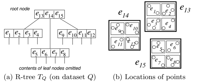
Figure 8: R-tree Example
