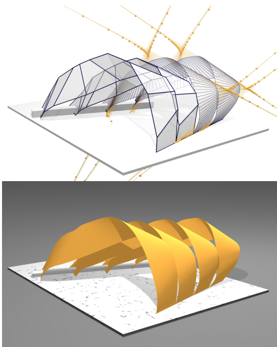
Figure 16: Design studies with developable surfaces. Two of four developable strips in the top figure show control structures, and the other two show the result of subdivision together with singular curves.
