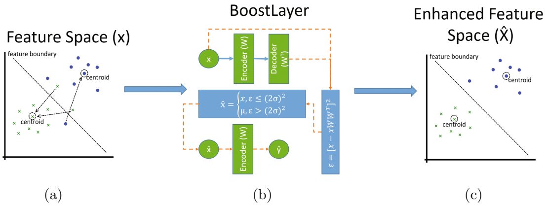
Fig. 2. Conceptualized diagram of our BoostLayer module. (a) The presence of outliers in the feature space impedes robust feature embedding. (b) The BoostLayer module detects outlier features based on a statistical properties. We use an orange dashed line to represent the outlier correction stage of the BoostLayer. For the sake of brevity, we did not include the biases and activation function in the diagram. (c) After correcting outliers, the intra-class feature variance is reduced, allowing for a more robust feature embedding.
