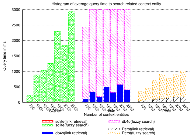
Figure 6. Breakdown of user experienced latency under various data size
