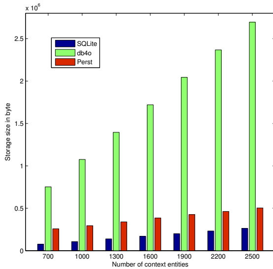
Figure 3. Storage consumption comparison
