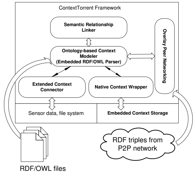
Figure 1. The Overview of ContextTorrent Framework
