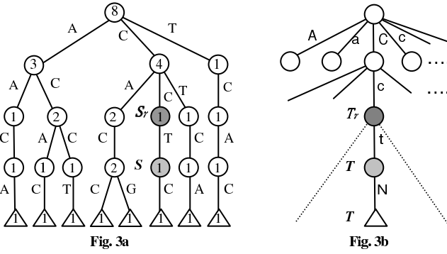
Fig. 3a. Suffix trie S (4-factor trie) for the sequence “AACACCTCACG” when l = 4 . e.g. node S_7 represents the substring “CC” and its child node S represents the substring “CCT” where the prefix of “CCT” is “CC”. Fig. 3b. Category tree T when l = 4 .
