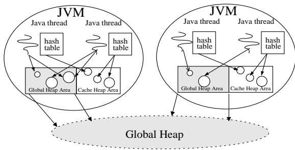
Figure 2. GOS architecture
