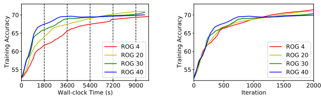
(a) Training accuracy against wall-clock time.
