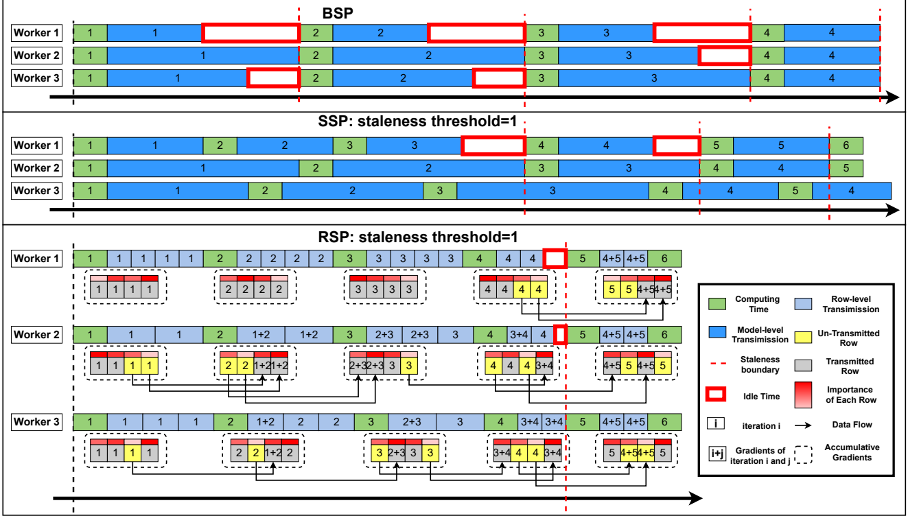
Figure 4: Workflow of ROG. The training model in RSP is divided into four rows and each row is synchronized in one row-level transmission. The bandwidth on these three devices are identical at the same time point in the three cases and the bandwidth is interfered by distance, occlusion, etc.
