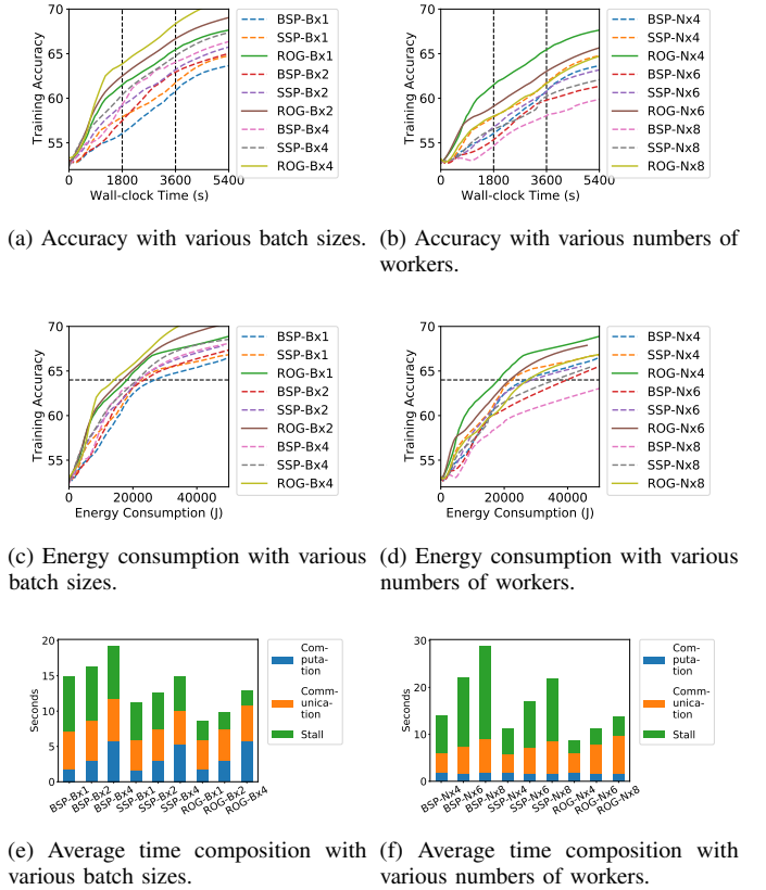
Figure 9: Sensitivity Studies about different batch sizes (left column) and worker numbers (right column)
