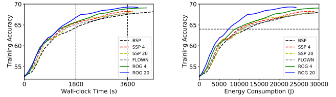
(c) Training accuracy against wall-clock time. (d) Energy consumption against training accuracy.
