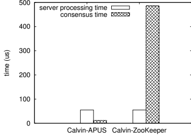
Figure 6: Comparing Calvin-APUS and Calvin-ZooKeeper.
