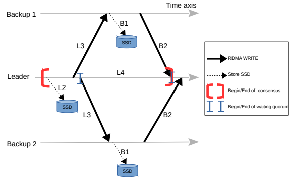
Figure 4: APUS consensus algorithm in normal case.
