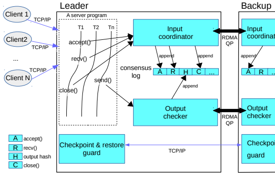
Figure 2: APUS Architecture (key components are in blue).
