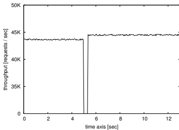
Figure 10: Redis throughput on APUS leader election.
