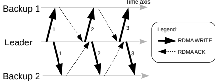
Figure 5: DARE’s RDMA-based protocol. It is a sole-leader, two-round protocol with three steps: (1) the leader WRITES a consensus request to all backups’ consensus logs and waits for ACKs to check if they succeed; (2) for the successful backups in (1), the leader does WRITES to update tail pointer of their consensus logs; and (3) on receiving a majority of ACKs in (2), a consensus is reached, the leader does WRITES to notify backups.
