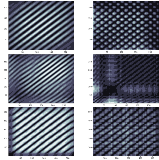
Fig. 18. Similarity map using L2 distance for each pair of motion frames comparing our learned phase manifold (left column) and pose/velocity features (right column), including a biped sprint (top), quadruped trot and canter (middle) and disco dancing motion (bottom).
