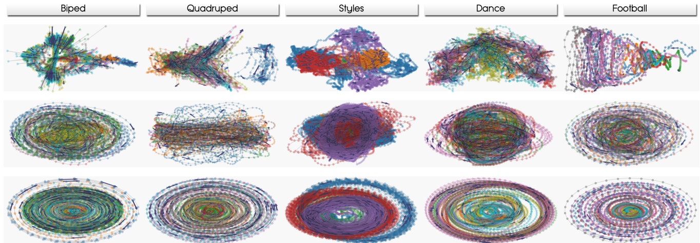
Fig. 6. Feature distributions for different motion domains in velocity space (top), latent space learned by convolutional + fully connected (middle) and phase space (bottom) visualized by 2D PCA projection. Each color represents poses from a single motion sequence that are temporally connected.
