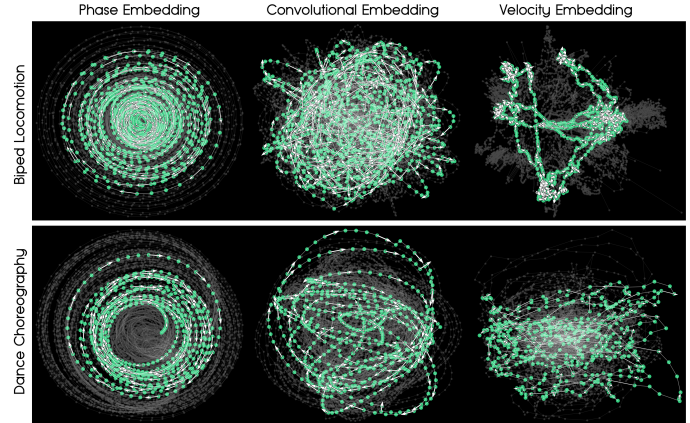
Fig. 7. 2D PCA embedding of the learned phase manifold compared to velocity and low-dimensional convolutional embeddings, highlighting the time series of a single motion clip of biped locomotion (top) and a dance choreography (bottom).
