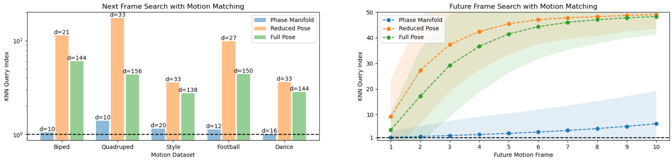
Fig. 15. The average index of the following frame in the motion capture data when matched with features of the phase manifold, reduced pose and full pose (left) and the average indices of the future frames in the motion capture data when matched with the three feature setups (right).
