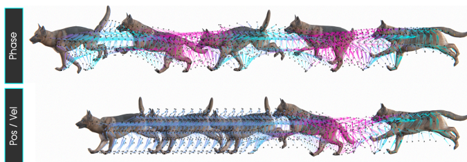
Fig. 17. Searching motions autoregressively into future by matching pose/velocity features (bottom) versus phase features (top). The color indicates the similarity of matched poses throughout the motion.
