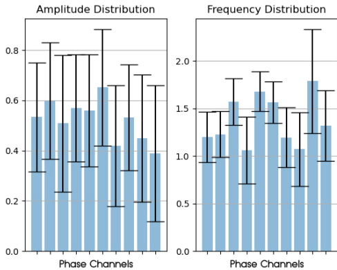
Fig. 4. Distribution of amplitudes and frequencies of learned phase channels. Each channel becomes tuned for a specific range of amplitudes and frequencies to decompose the motion, roughly acting like a set of learned band-pass filters. Note that there were no parameter ranges predefined for each phase channel, but they are extracted as needed by the model.
