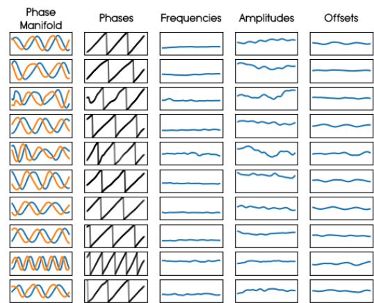
Fig. 3. Learned parameters for phase, amplitude, frequency and offset for a fixed window of motion during network training to reconstruct the input motion, and from which the phase manifold can be constructed.
