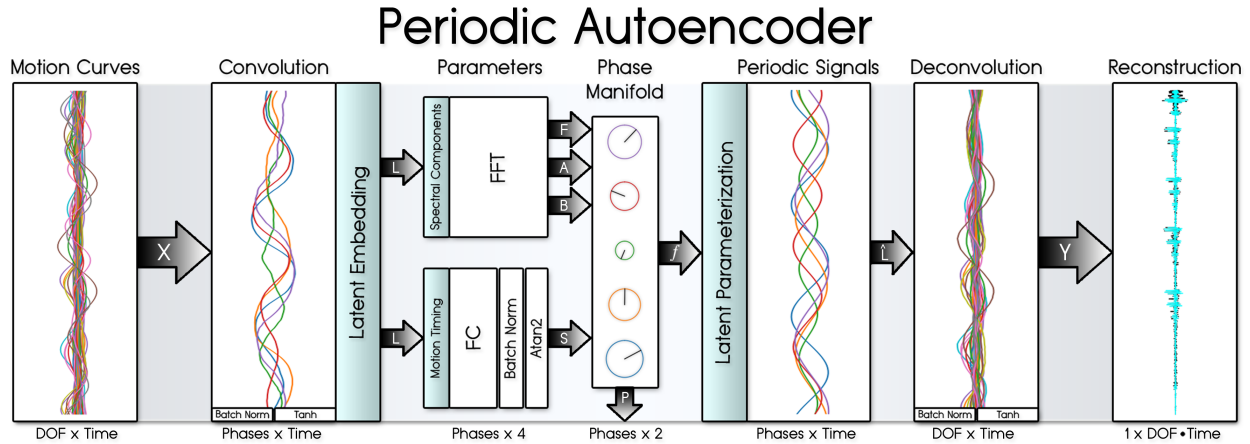
Fig. 2. Network architecture of the Periodic Autoencoder for extracting multi-dimensional phase manifolds from unstructured motion data.
