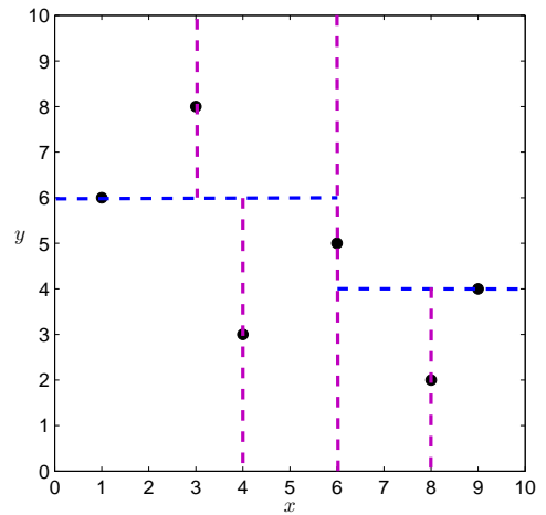
(a) KD-tree-based partitioning
