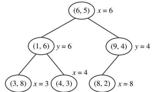
(b) KD-tree structure
