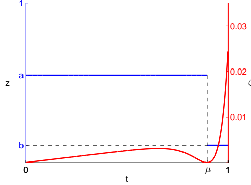
Fig. 1: Primal z and Dual \zeta
